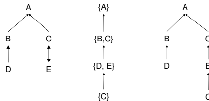
Figure 1. In the middle, a single terminated argument game based on the defeat graph on the left, and its reply graph on the right.
