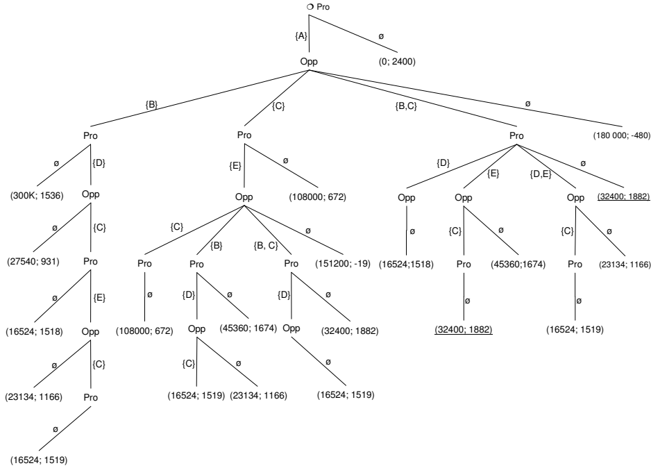
Figure 2. An extensive game tree. The payoffs for the Proponent and Opponent are indicated for each terminal game in terms of expected utility (see Section 4). Underlined payoffs correspond to the perfect equilibria.
